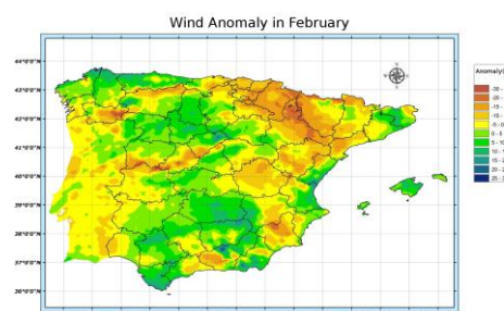
Fig 4. February wind anomalies in Spain. Source: CENER
