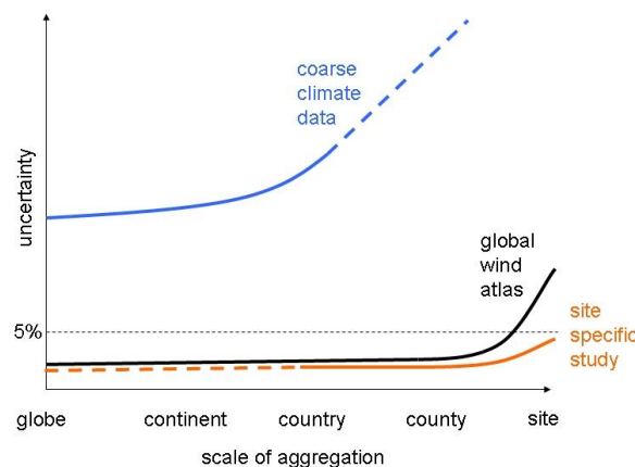
Figure 6: Uncertainty of wind resource data as a function of different scales of aggregation. Schematic graph illustrating the uncertainty of wind resource data as a function of different scales of aggregation. The horizontal axis gives scale of aggregation, decreasing from left to right, from global to turbine site scales. The vertical axis gives uncertainty and a value of 5% is given as reference level of uncertainty. The expected uncertainty is given for three methodologies. The ‘coarse climate data’ represents the current source of global resource estimation used by global energy planners. The ‘site specific study’ represents state of the art resource studies conducted by, among others, commercial companies. The ‘global wind atlas’ represents the methodology designed to optimize usefulness for global energy planners whilst being economical to produce
