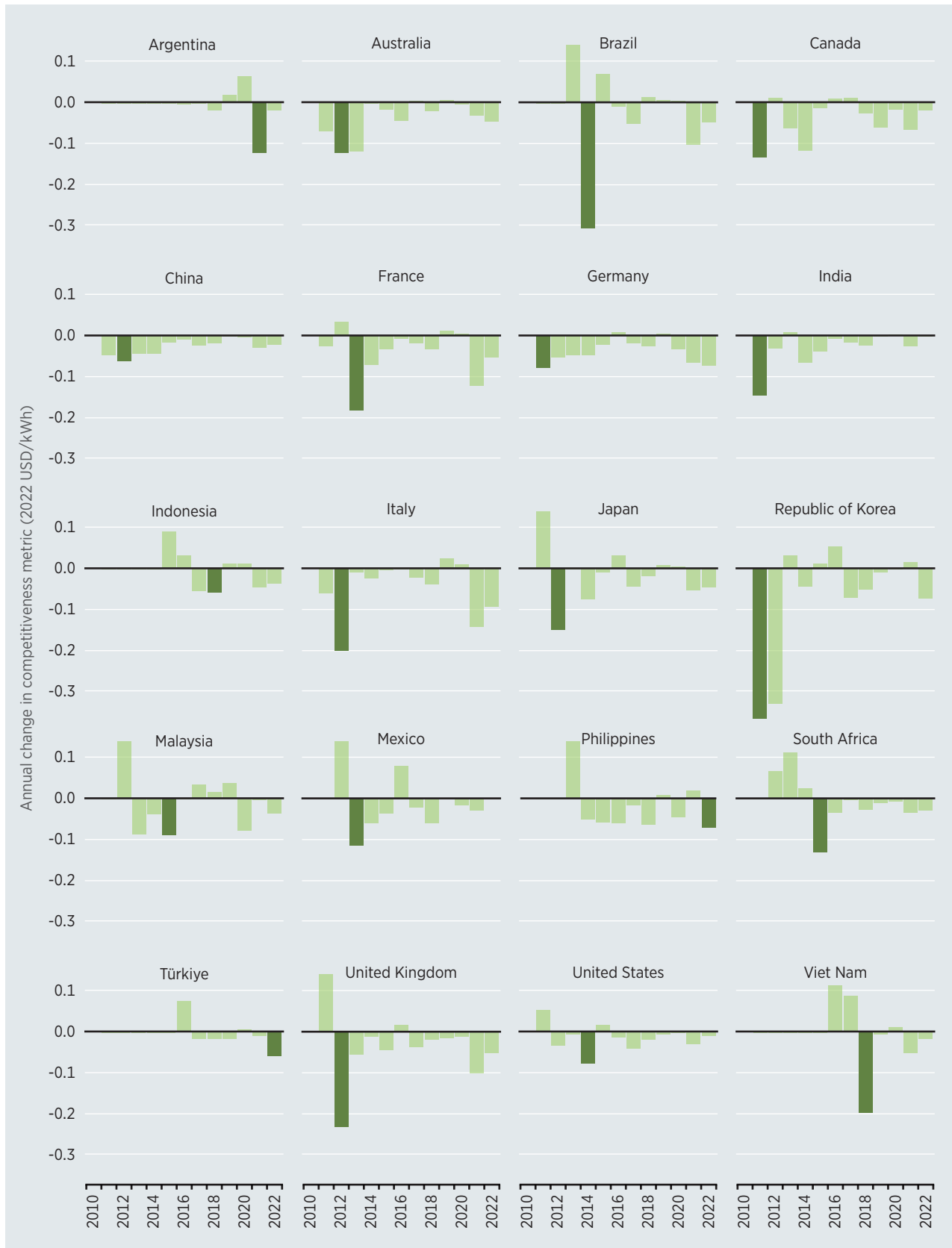
Figure 1.8 Annual change in competitiveness of new utility-scale solar PV capacity added by country and year, 2010-2022
