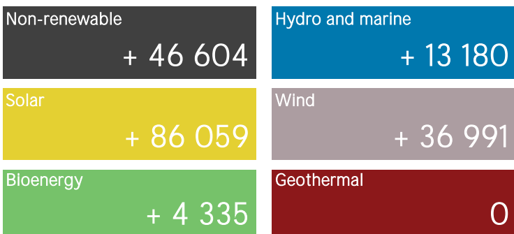
Net capacity change in 2022 (MW)
