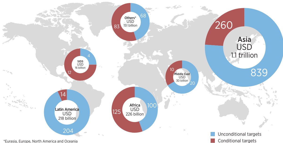
Figure 1 Total investment needed by 2030 for the implementation of renewable energy targets in current NDCs (USD billion)
